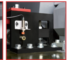
Over Thickness Safety Device
